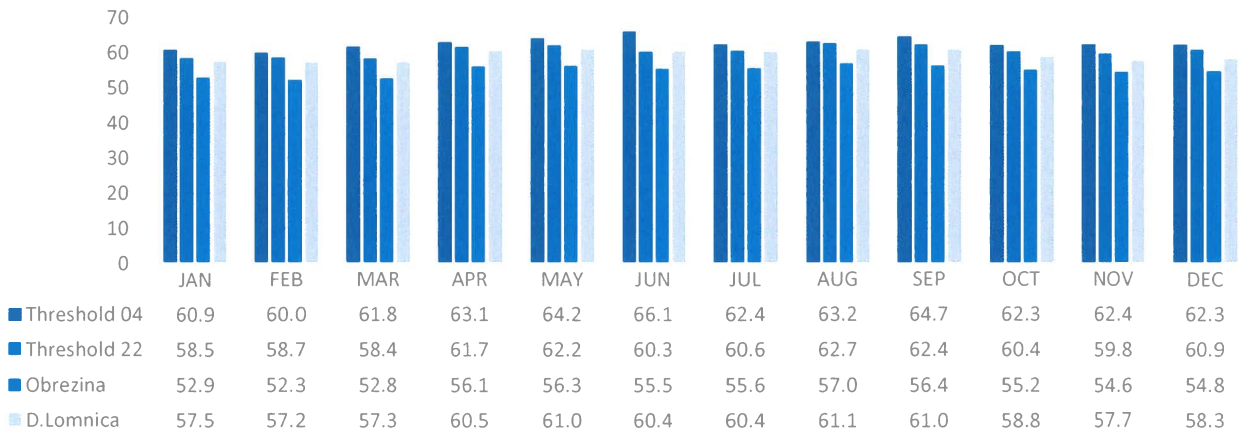
Noise measuring results from Jan 2023 - Dec 2023
